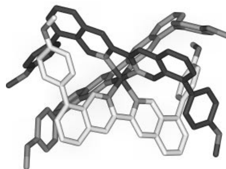
Figure 2. Crystallographic structure of the [\text{Fe}(\text{I})_3]^{2+} cation 41 .
